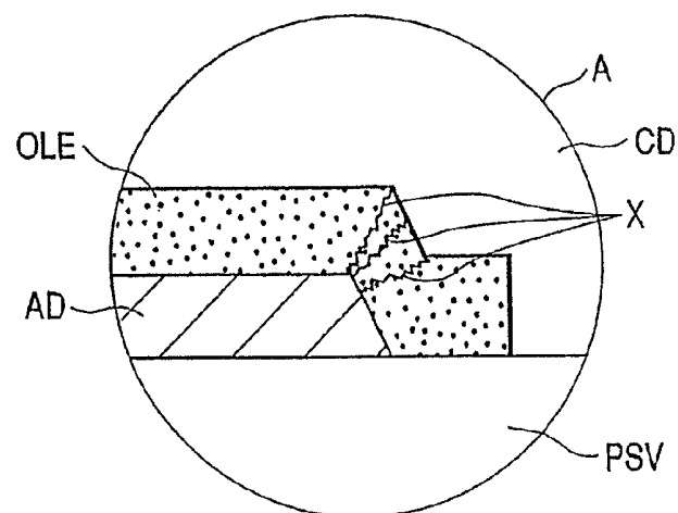
FIG. 16 (PRIOR ART)
