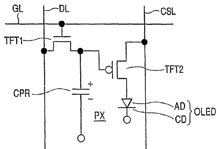
FIG. 13 (PRIOR ART)
