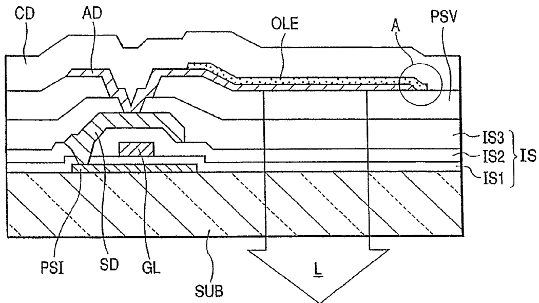
FIG. 15 (PRIOR ART)
