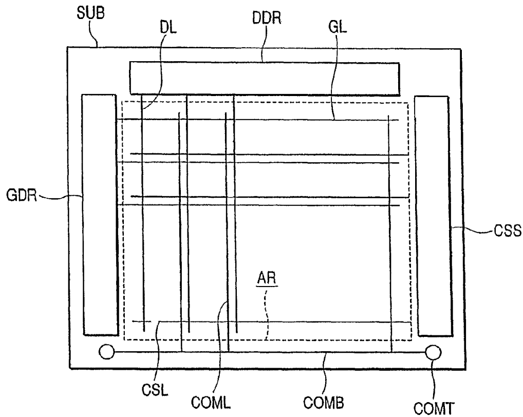
FIG. 12 (PRIOR ART)
